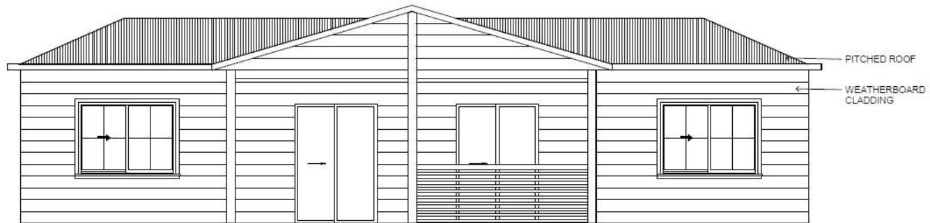
FRONT VIEW
